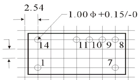
DIP 14 封裝
