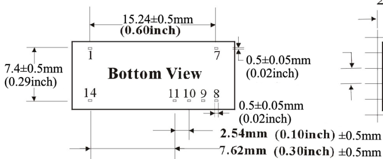
DIP 14 封裝
